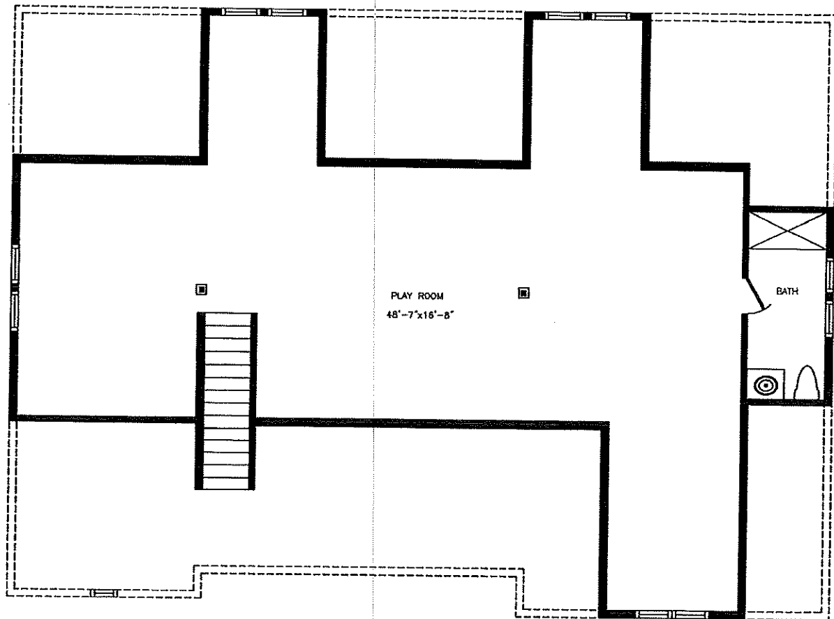
ATTIC PLAN
